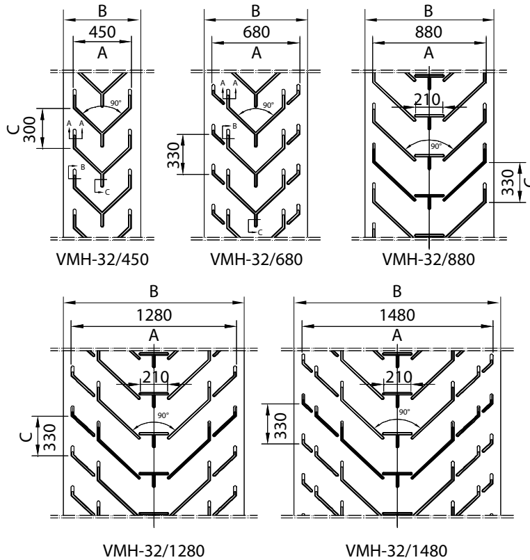
Profile shape B-B
