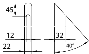
Profile shape B-B
