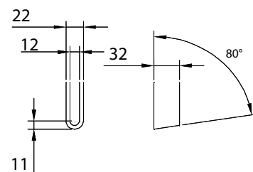
Profile shape C-C
