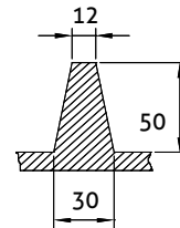
Cross section A-A
