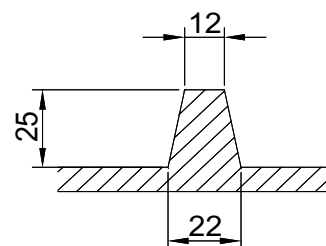
Cross section A-A
